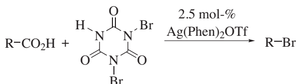
Figure 18: Decarboxylative Bromination
