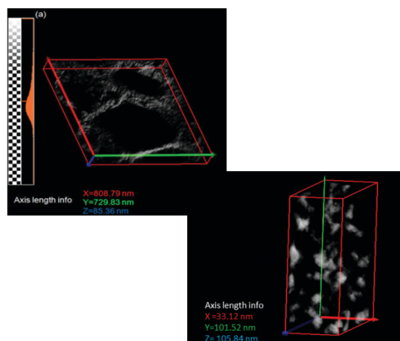
Figure 3. 3D -TEM images of natural rubber with
