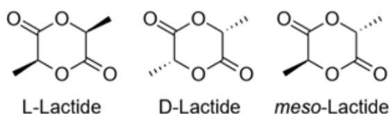
Figure 2: Stereoisomers of lactide
