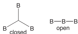
Figure 3: Closed and open \text{B}_3 units
