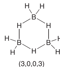
Figure 4: Topological structure of B 3 H 9
