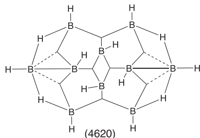
Figure 10: Most preferred topology of B_{10}H_{14}
