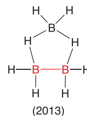
Figure 11: Topological structure of [B_3H_8]^-
