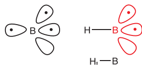
Figure 2: sp^3 -hybridised-B and \text{H}_t -B bond
