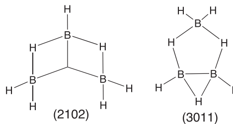
Figure 7: Possible topologies for B_3H_7
