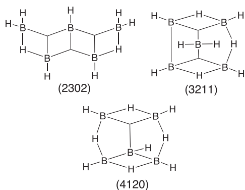
Figure 8: Topological structures of B_5H_9
