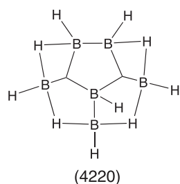
Figure 9: Most preferred topology for B_6H_{10}
