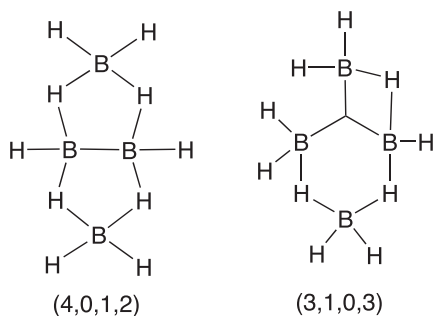
Figure 5: Possible topologies for B_4H_{10}
